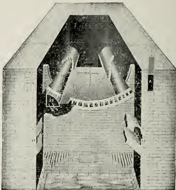
TYPICAL SETTING FOR RETURN TUBULAR BOILERS.
